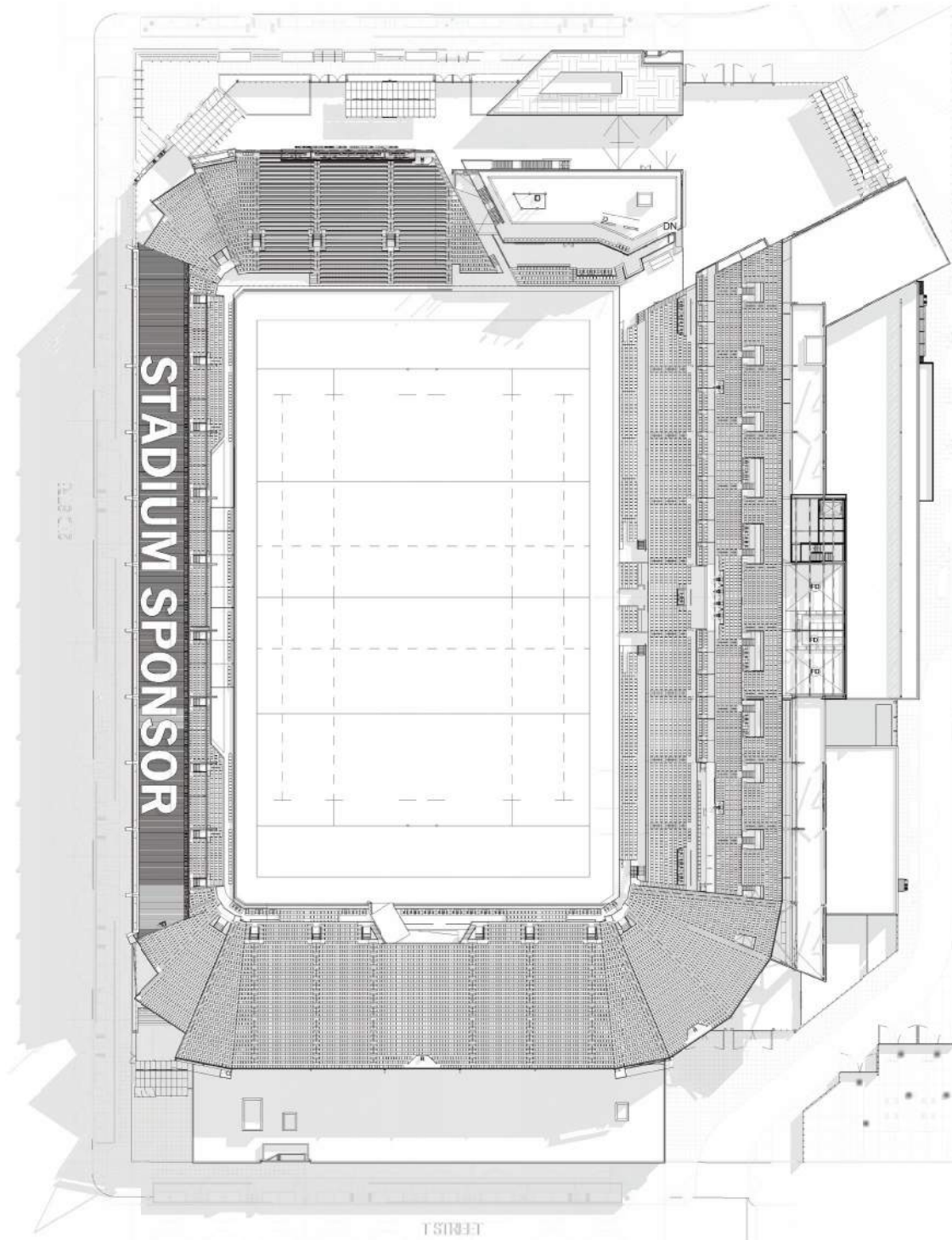
1 RUGBY FIELD LAYOUT 1" = 50'-0"
